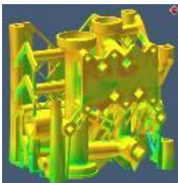
Simufact-GR-Simufact-AM-manifold-effective-stress.jpg
