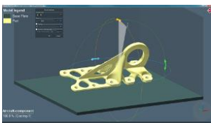
Simufact-GR-aircraft-component-positioning-rotation.jpg
