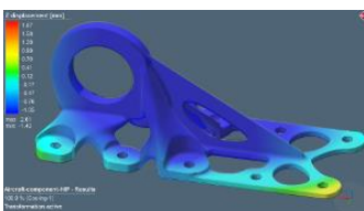
Simufact-GR-aircraft-component-transferredResults.jpg
