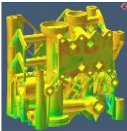
Simufact-GR-Simufact-AM-manifold-effective-stress.jpg
